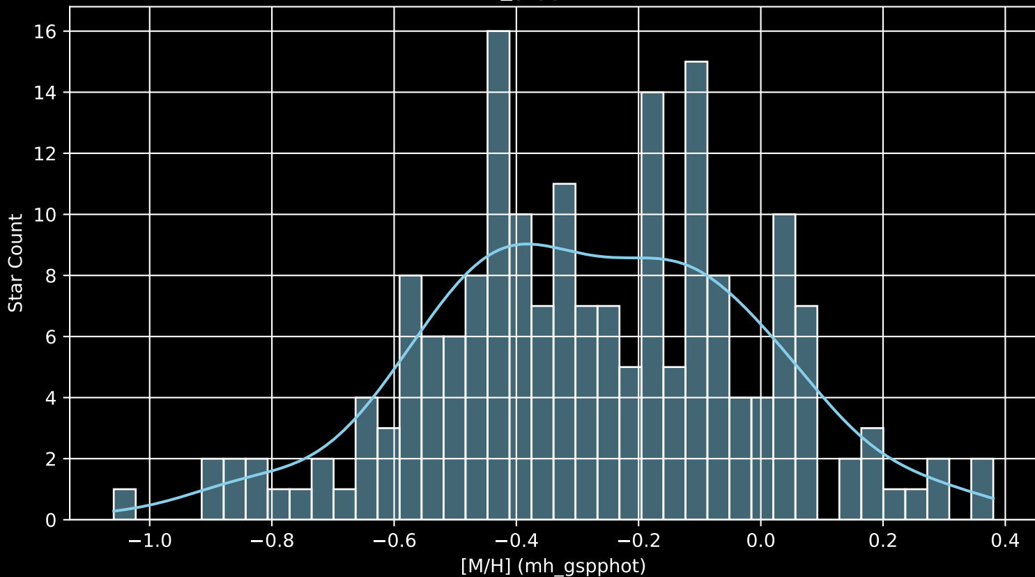
GALAH DR4 Field: [7130] [M/H] (mh_gspphot) (n= 188)
