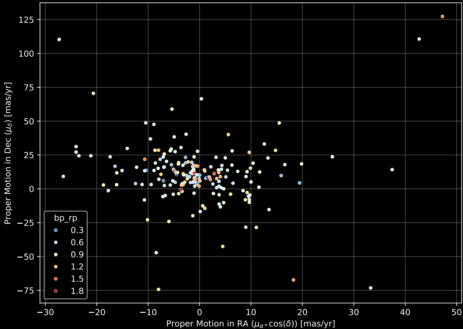
GALAH DR4 Field: [7130] Proper Motion Diagram (n= 189)
