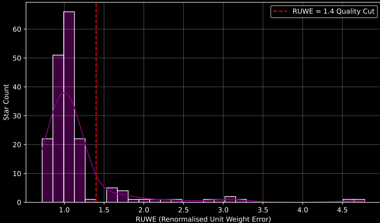
GALAH DR4 Field [7130] RUWE Distribution (n= 183)
