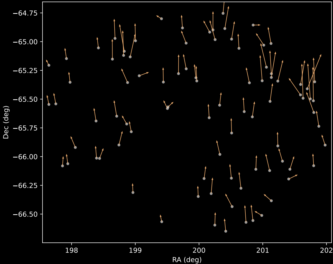
GALAH DR4 Cluster 3 Proper Motion Vectors (n=88)
