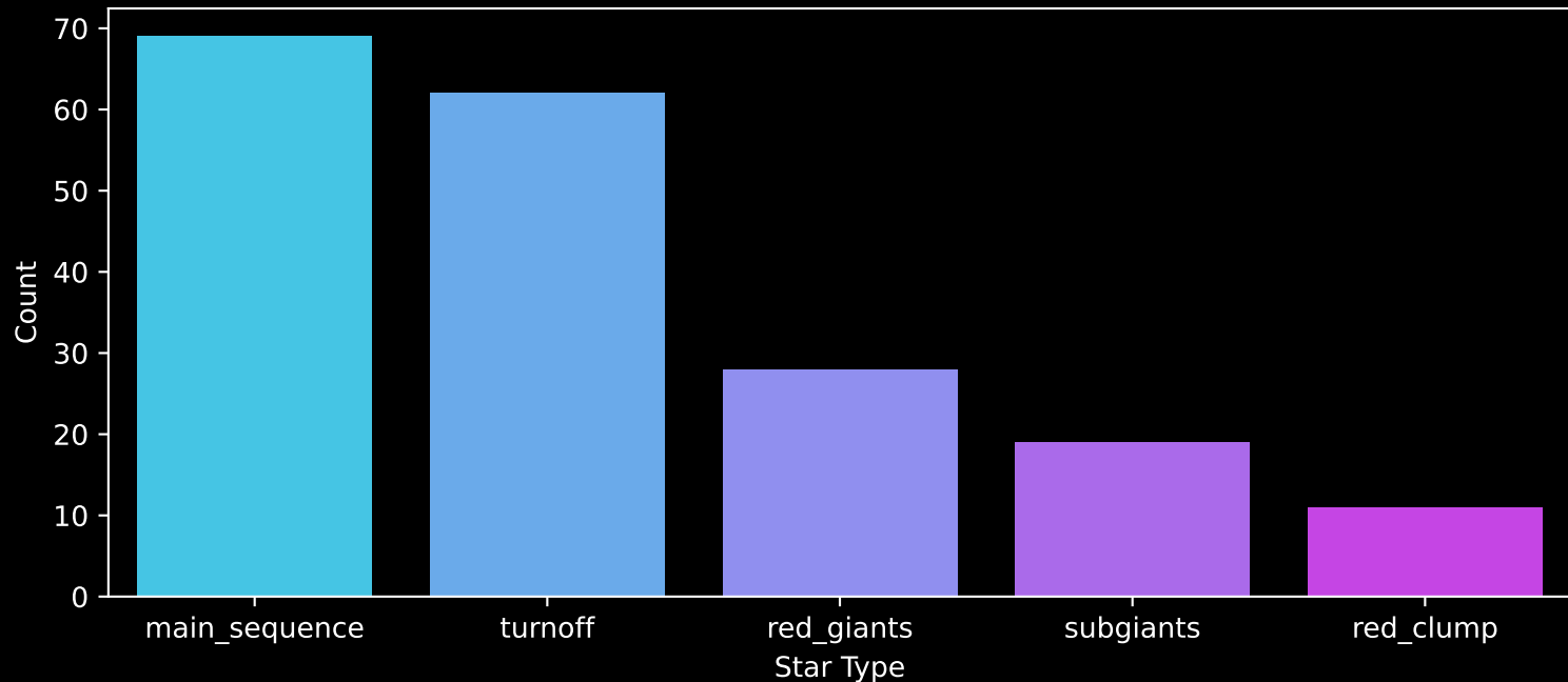
GALAH DR4 Field: [7130] Count plot of Star Type
